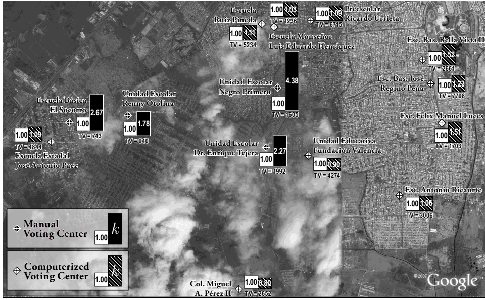
Figure 16: Partial aerial view of Miguel Peña township (taken from Google Earth). Manual vs. computerized voting centers are compared in regards to their k value and total number of votes (TV). The image is centered at Latitude 10^{\circ}7'32.66'' N and Longitude 68^{\circ}1'22.48'' W.
