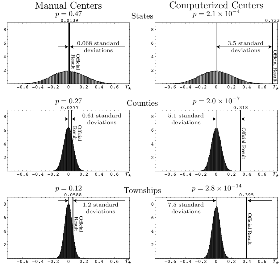
Figure 20: Comparison of official results correlation r_* vs. expected value distribution found after 100,000 simulations for manual and computerized centers at state, county or township level. The simulation results follow a normal distribution, which is shown as a dotted line. The probability of the official r_* happening by chance is indicated as p .
