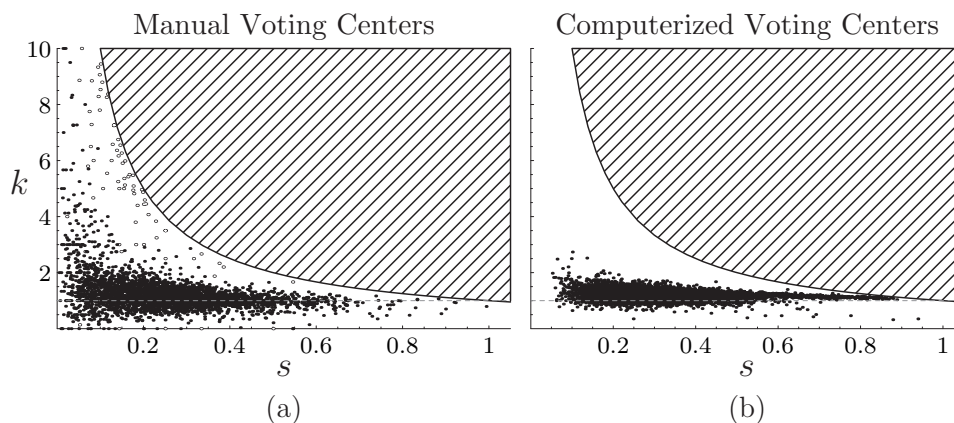
Figure 3: Relationship between k and s for computerized and manual centers. The shadowed area contains the mathematically impossible values of k . The maximum k value is 1/s . The hollow dots represent voting centers located in consular offices.
